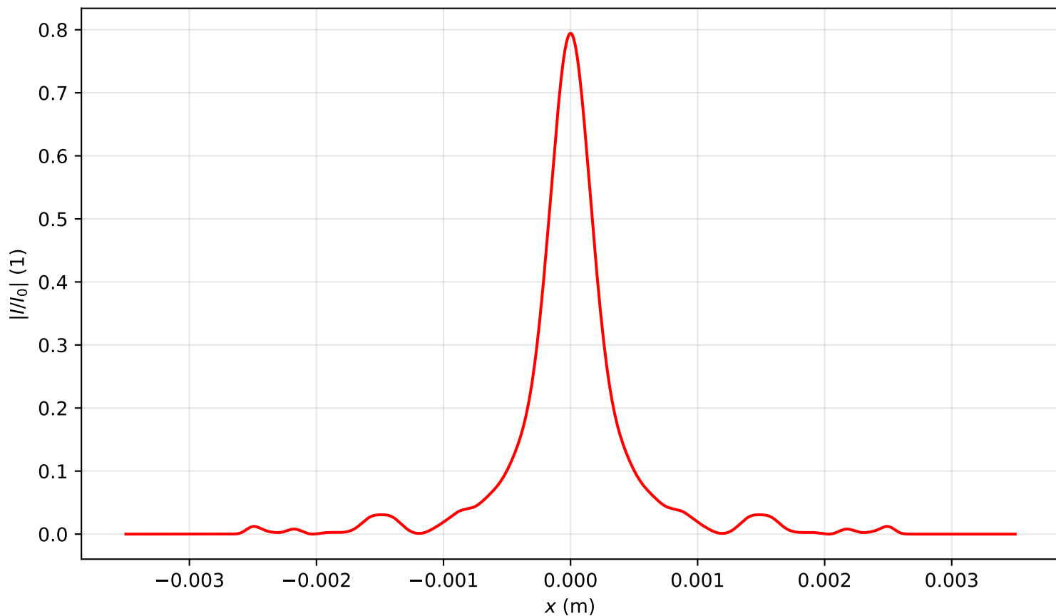
Intensity profile I(x, y = 0, z = 2.866)/I_0 , \text{Pin}=4.0\text{Pcr} , artificial time
